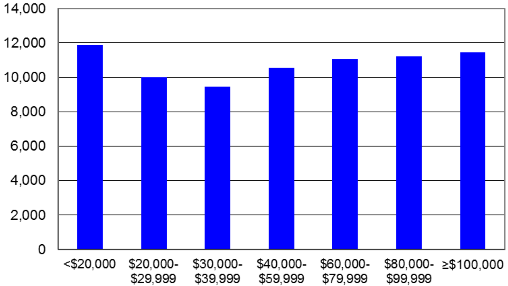
Figure 3: Average steps by household income, Ontario
