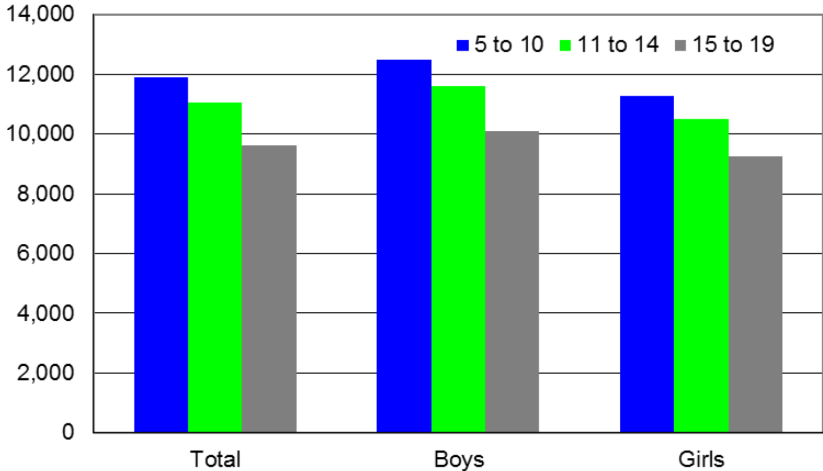
Figure 2: Average steps by age and gender of child, Ontario
